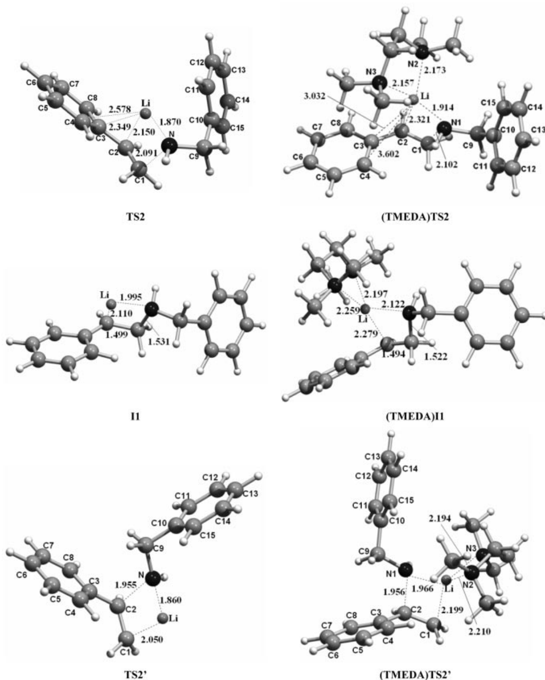
Figure 4. Transition states [TS2 and (TMEDA)TS2] of the anti-Markovnikov nucleophilic attack of the lithium amide on styrene (top) as well as the resulting anti-Markovnikov intermediates [II and (TMEDA)II] formed in this attack (center). The transition states for the Markovnikov nucleophilic attack [TS2' and (TMEDA)TS2'] are depicted in the bottom row (all interatomic distances in Å).
