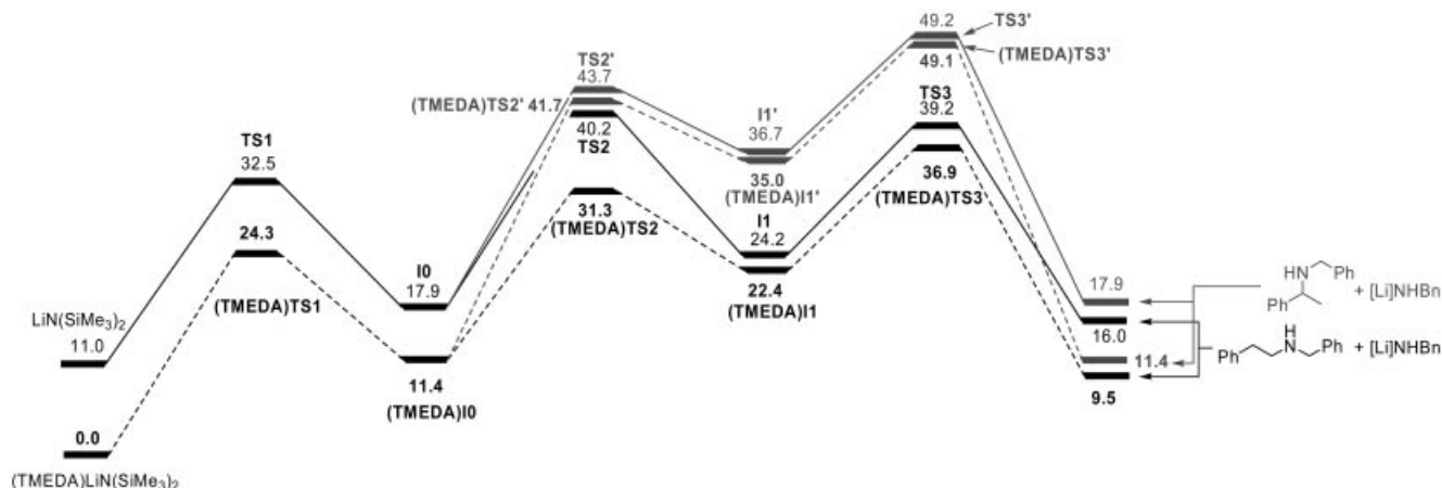
Figure 2. Gibbs energy profile in benzene solution for the catalytic anti-Markovnikov hydroamination of styrene with benzylamine, catalyzed by LiN(SiMe_3)_2 (solid line) or (TMEDA)LiN(SiMe_3)_2 (dashed line). The relative Gibbs energies at 298.15 K and 1\text{ mol L}^{-1} in \text{kcal mol}^{-1} are given. The corresponding profile for the Markovnikov addition is given in grey.
