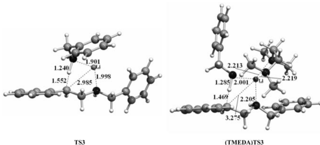
Figure 5. Transition states [ TS3 and (TMEDA)TS3 ] for the lithium/proton exchange between II and (TMEDA)II , respectively, and benzylamine in the absence (left) and presence of TMEDA (right). Interatomic distances are given in \text{\AA} .
