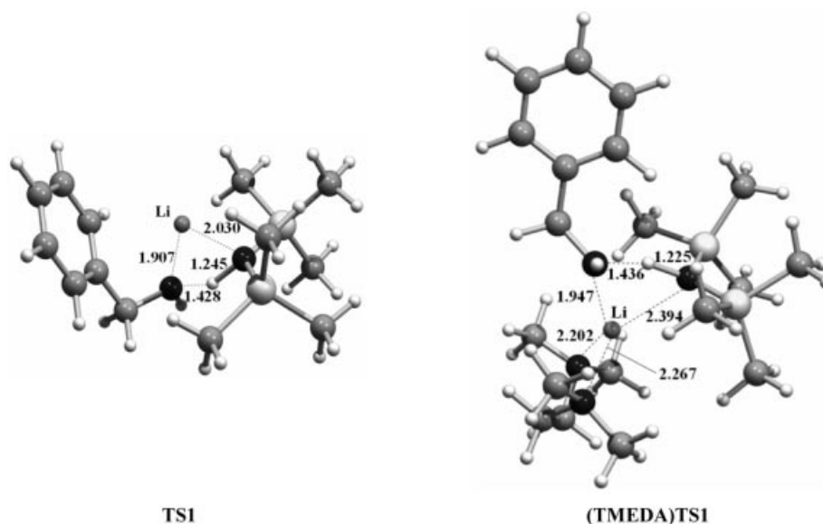
Figure 3. Transition states [TS1 and (TMEDA)TS1] for the lithium/proton exchange between LiN(SiMe_3)_2 and benzylamine in the absence (left) and presence of TMEDA (interatomic distances in Å).
